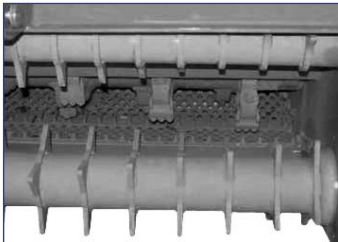
Knives, screen, re-cutter bar and lower pick-up rotor
